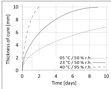
Diagram 1: Curing speed Sikasil® WS-300 KR
