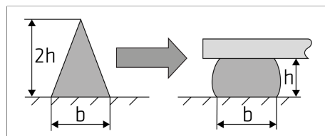
Figure 1: Recommended bead configuration
