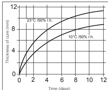
Diagram 1: Curing speed for Sikaflex® -211 EN
