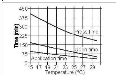
Diagram 1: Open time, press time and application time for SikaForce®-7720 L105
