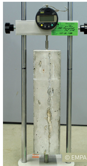
The increase in volume due to the strain resulting from ASR becomes perceptible by measurement of a change in length of test specimens. Ordinarily the specimens are stored under intensified conditions (temperature, humidity, applied load) in order to accelerate the reaction.
