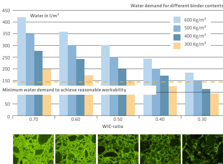
Figure 2: The water reduction potential to increase durability must be compatible with the placing practicalities
