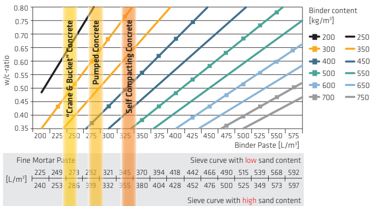
Figure 5: Relation between concrete compressive strengths of a specific cement, expressed in w/c-ratio, and the fine mortar quantity (L/m 3 ) for a required cement content (kg/m 3 )
