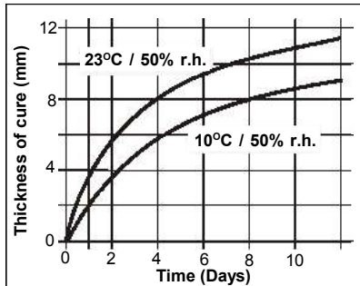
Diagram 1: Curing speed for Sikaflex®-221
