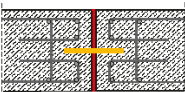
EXPANSION JOINT WATERSTOP, INTERNAL
