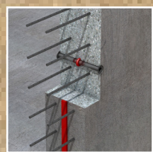
Construction joint
